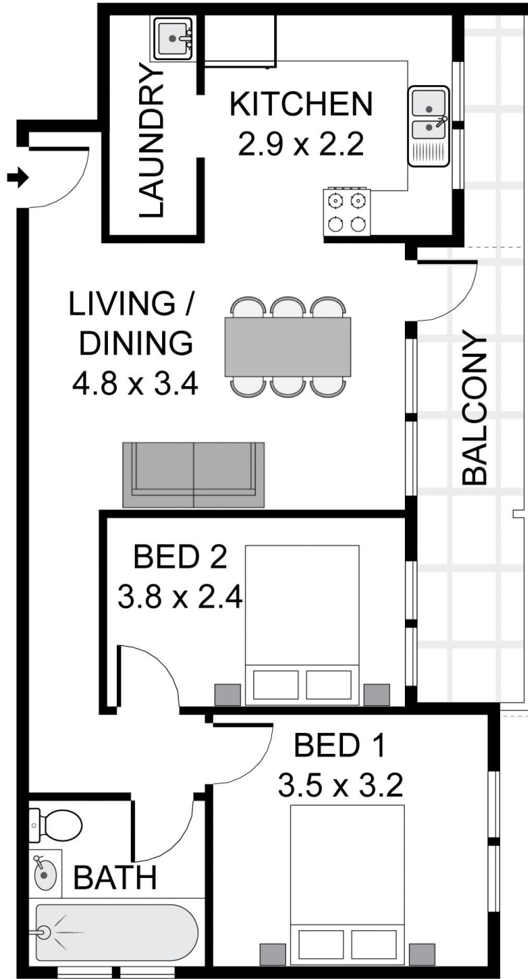
TOP FLOOR
