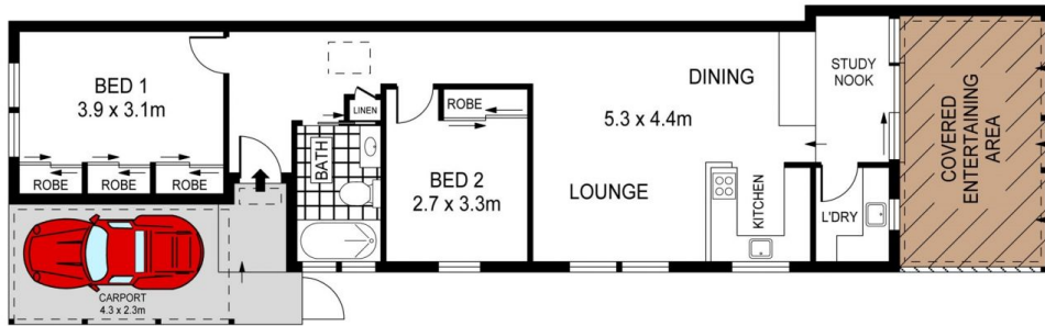
GROUND LEVEL
