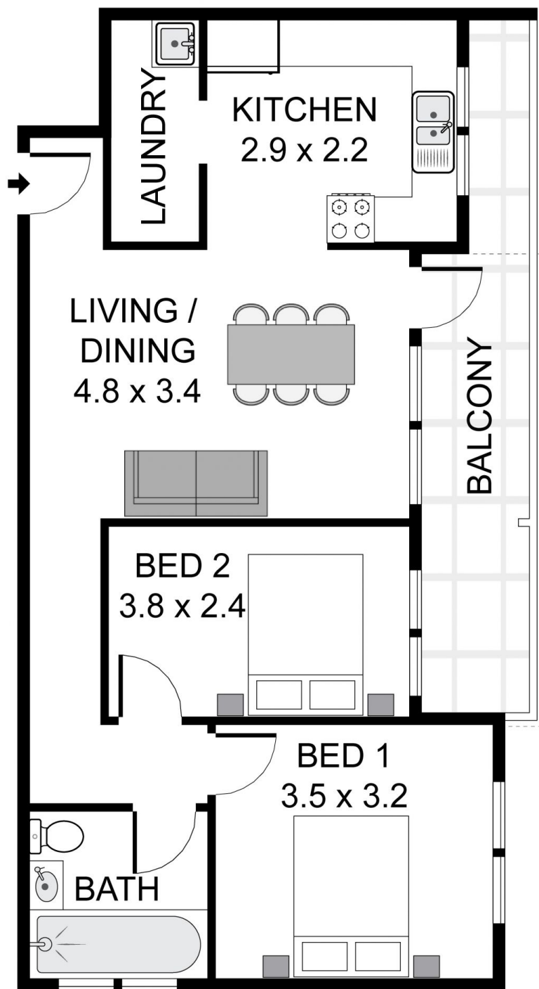
TOP FLOOR
