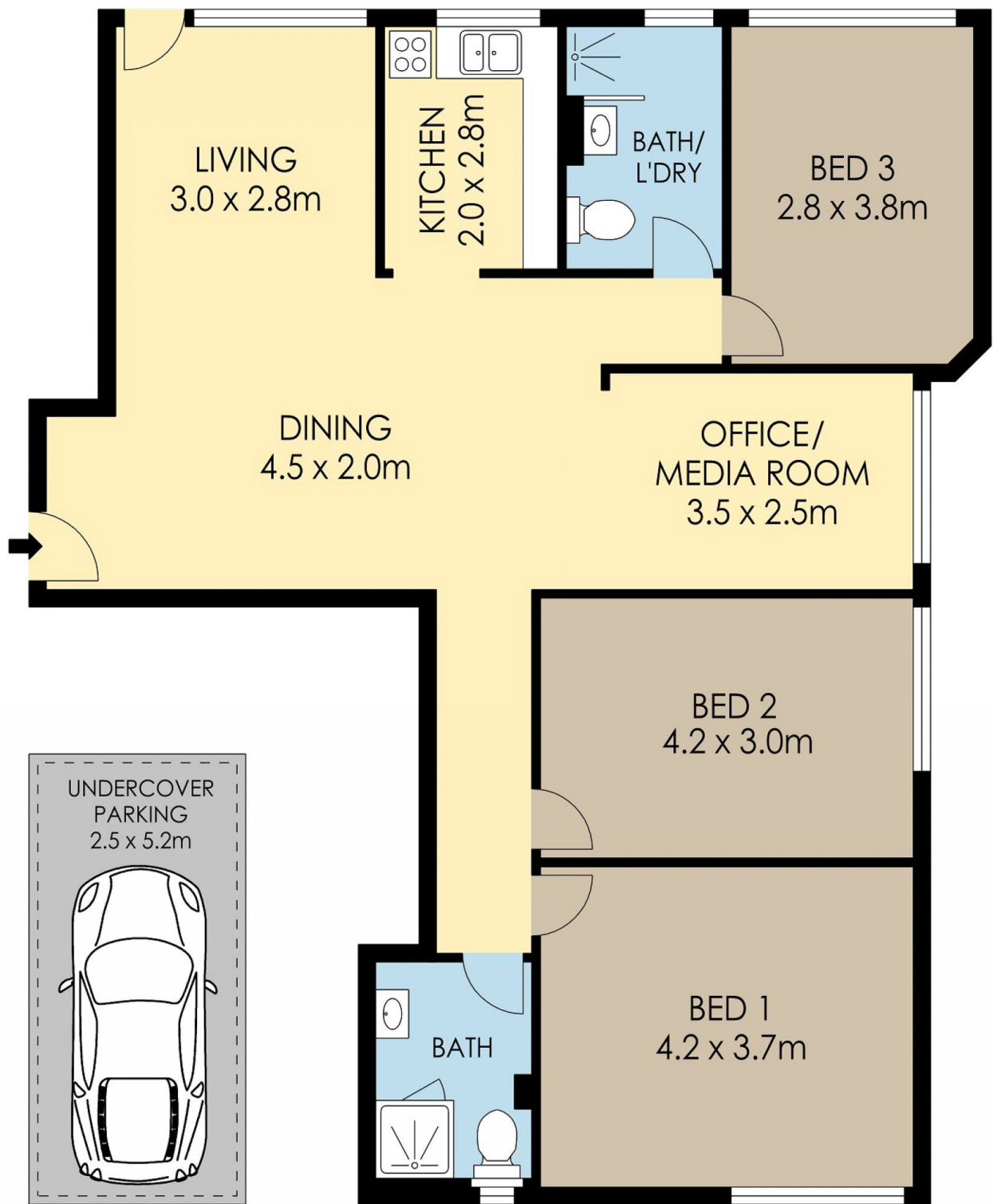
GROUND LEVEL
