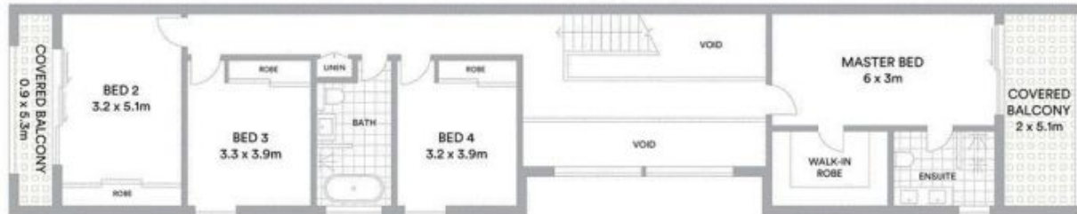
FIRST FLOOR
