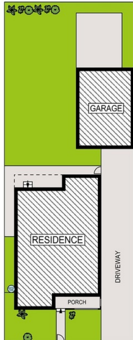
SITE PLAN
