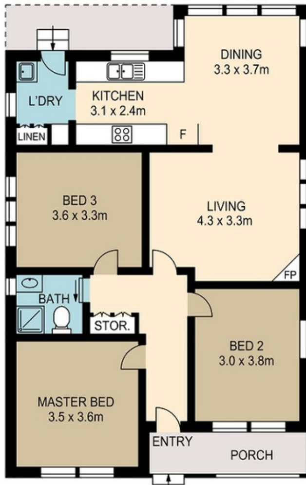
FLOOR PLAN
