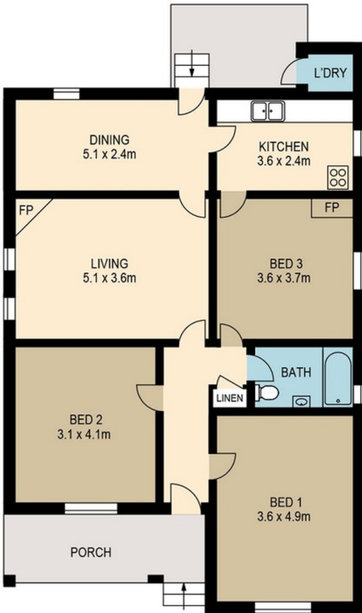
FLOOR PLAN
